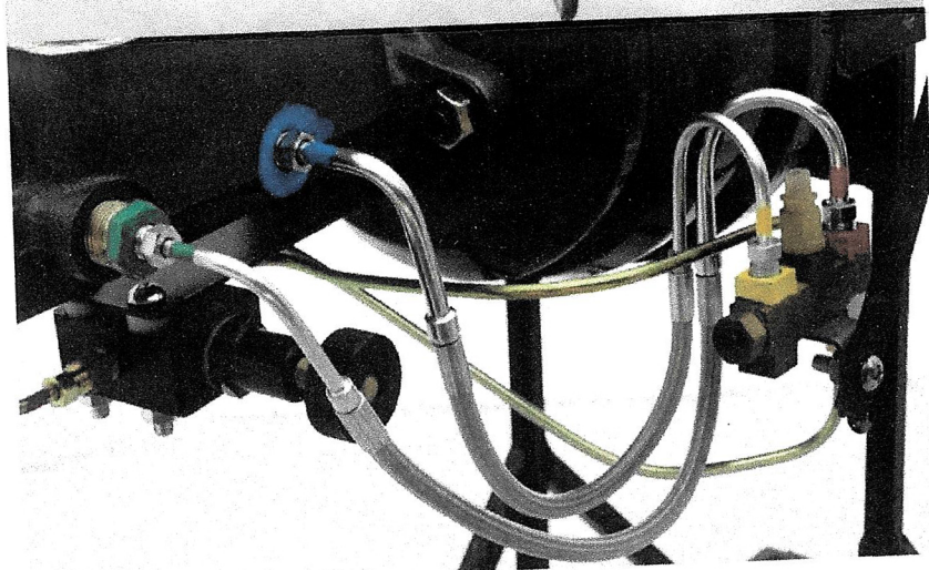
LINE KIT FOR CSRPOWER BRAKE KIT ON 67-69 MUSTANG
